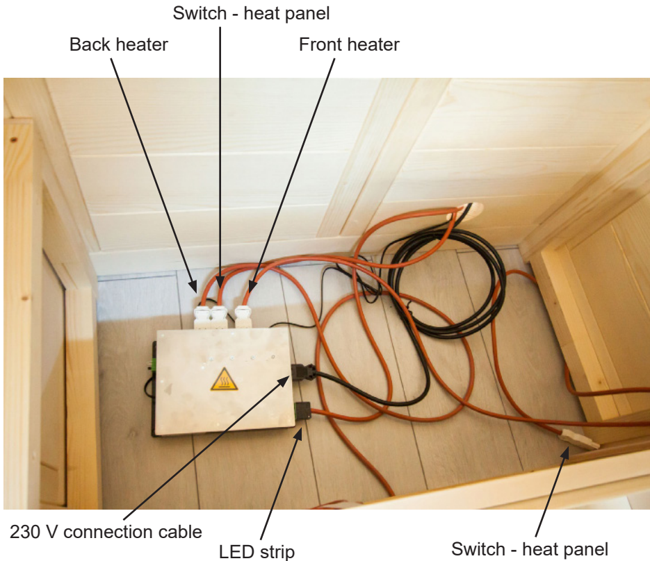
Fig. 25: Example for connection
